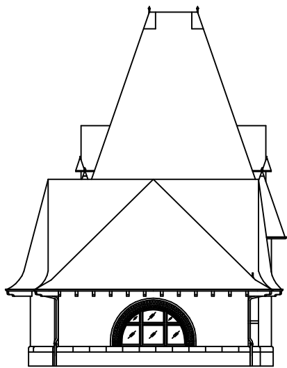
NORTH ELEVATION
